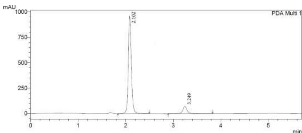
Figure 3: Standard chromatogram
