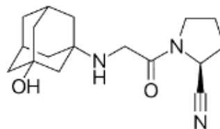
Figure 2: Structure of Vildagliptin
