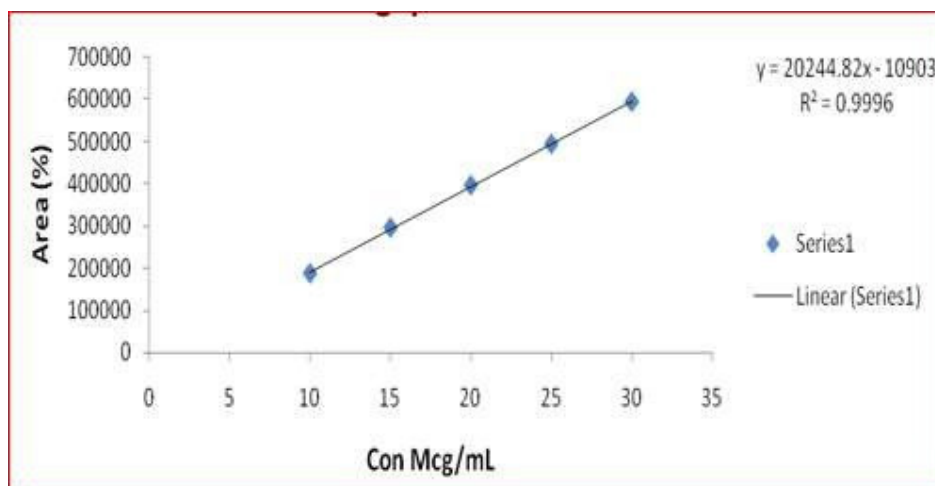
Figure 7: Linearity graph for Vildagliptin
