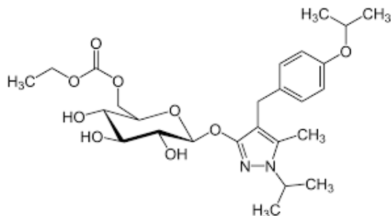
Figure 1: Structure of Remogliflozin Etabonate
