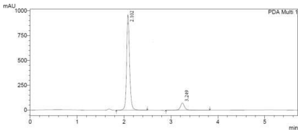
Figure 4: Sample chromatogram
