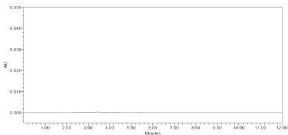
Figure 5: Blank chromatogram
